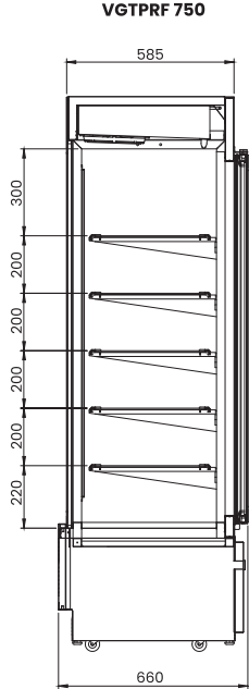
VITRINE GLASS TOWER PREMIUM PRATELEIRA FIXA 750
